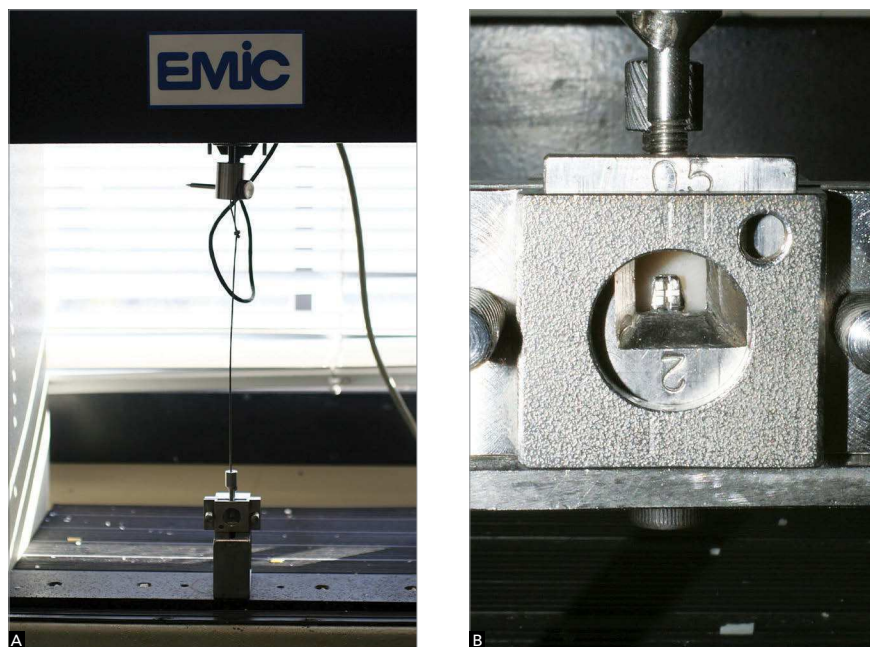
Figure 2 - A) shear bond strength test, B) specimen positioned in the testing machine
